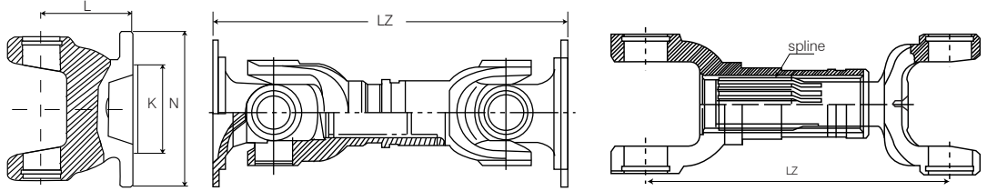
DRIVESHAFTS / SHORT COUPLE SETS
