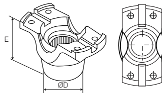
END YOKES
