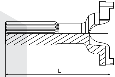
YOKE SHAFT
