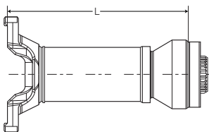
SLIP SETS
