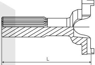
YOKE SHAFTS
